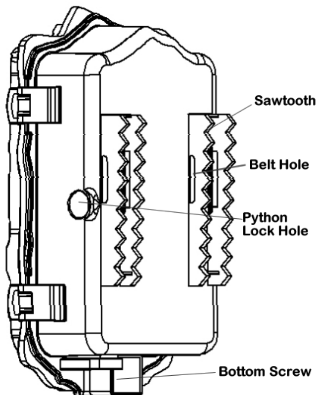
Fig. 6: The back panel of the camera
