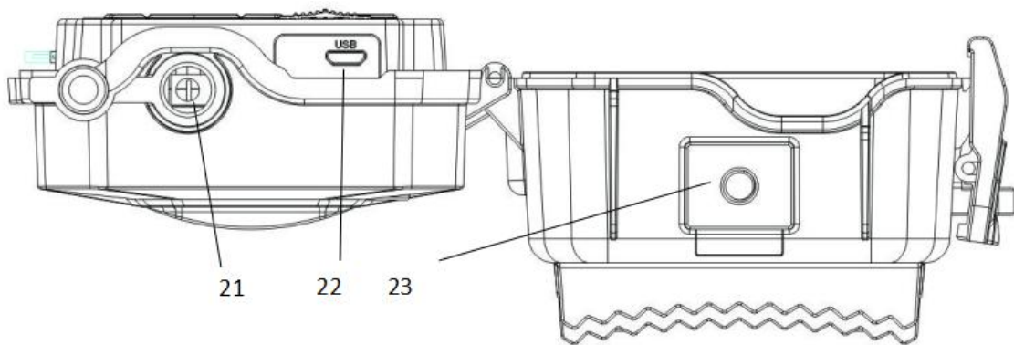
Fig. 3: Bottom view
